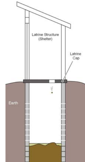
Figure 33: Latrine Example
